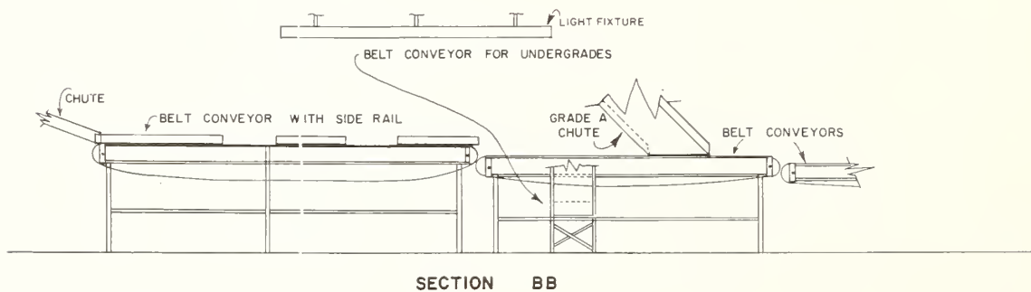
Figure 8.--Layout of turkey grading area in plant D.
